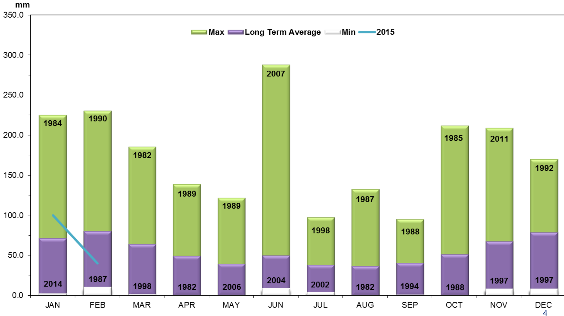
Rainfall Pattern and History (1981 - 2015)
