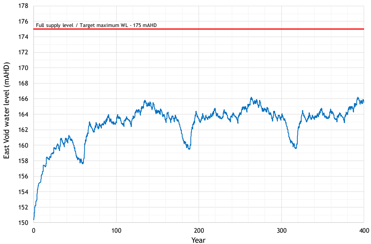
Figure 7.4 - Final void water levels - East Void
